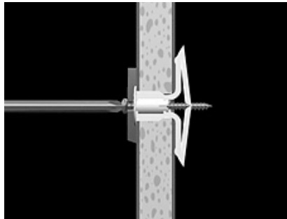
Photo E - Place item over anchor. Insert screw and tighten until screw is flush with fixture. Then, stop. The anchors also wedge securely in thick or solid walls, or in wood studs behind drywall.
