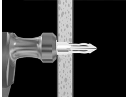
Photo C - Insert anchor in hole and tap flush with wall.
