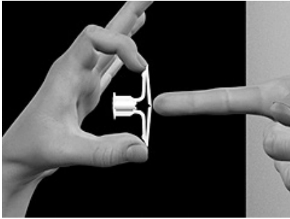
Photo B - Drill 5/16" diameter (8mm) hole. Fold anchor in middle.
