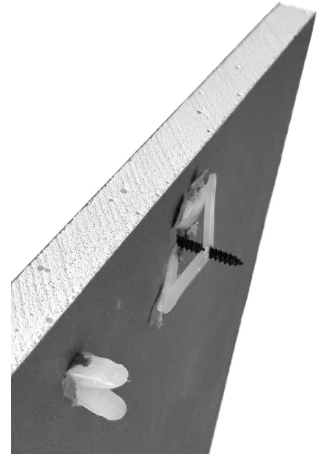
Photo F - correct (top) and incorrect (bottom).
