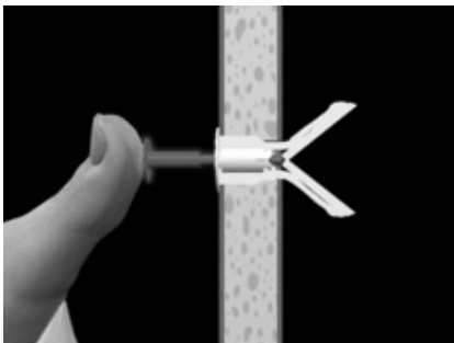
Photo D - Insert key to pop anchor open & lock behind hollow wall (not necessary for thick or solid walls). Do not force of hammer key.
