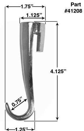
Photo B - Pan Hook
